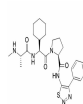
Chemical structure of GDC-0152
