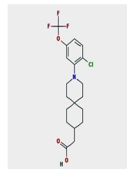
Chemical structure of GPR120 Compound A
