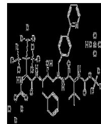
Chemical structure of CTP 518(Atazanavir...)
