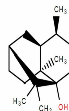
Chemical structure of Patchouli Alcohol
