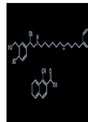
Chemical structure of Salmeterol Xinafoa...
