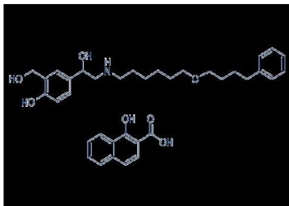
Chemical structure of Salmeterol Xinafoate
