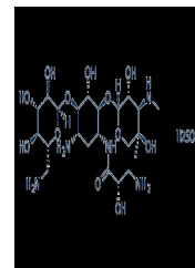
Chemical structure of Isepamicin Sulphate...
