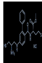
Chemical structure of FTI 277 HCl
