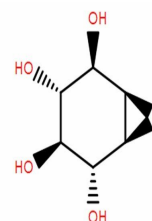
Chemical structure of Conduritol B Epoxi...
