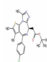
Chemical structure of (-)-JQ-1
