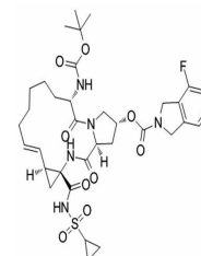
Chemical structure of Danoprevir (RG7227...)
