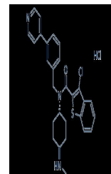
Chemical structure of SAG
