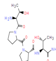
Chemical structure of Rapastinel(GLYX-13...)
