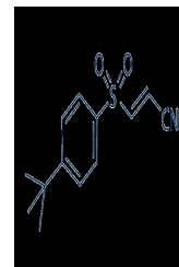
Chemical structure of Bay 11-7085
