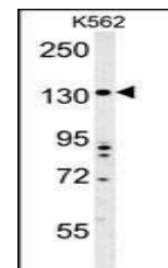
Western Blot of K562 cell line lysates u...
