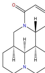
Sophocarpine
