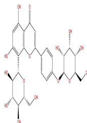
Glucosylvitexin
