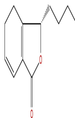
Senkyunolide A
