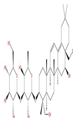
Saikosaponin B1
