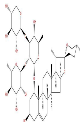
Ophiopogonin D
