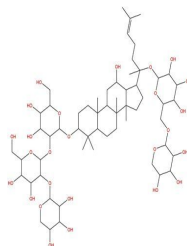
Notoginsenoside Fc
