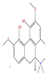
Magnoflorine Iodide
