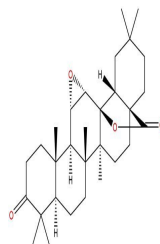
Liquidambaric lactone
