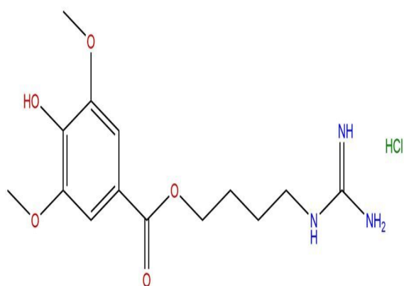
Leonurine Hydrochloride
