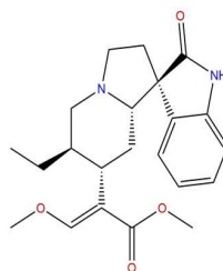
Isorhynchophylline
