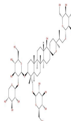
Hosenkoside M
