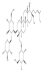
Hosenkoside G
