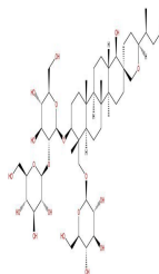
Hosenkoside A
