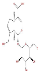
Geniposidic acid
