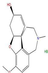
Galanthamine hydrobromide
