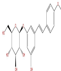
Desoxyrhaponticin
