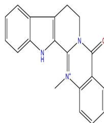
Dehydroevodiamine hydrochloride
