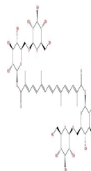
Crocin I
