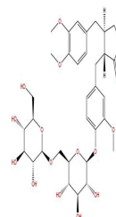
Chemical structure of Arctigenin 4'-O-be...
