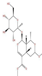
7-O-Methyl morroniside
