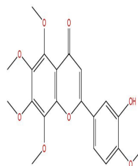
Chemical structure of 3'-Demethylnobiletin...
