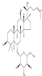
20(R)- Ginsenoside Rh1
