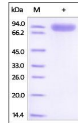
SDS-PAGE analysis of Mouse ROR1 protein
