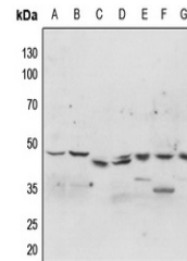
Western blot analysis of p47 phox (Phosp...
