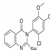
Chemical structure of Mdivi-1
