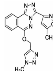
Chemical structure of alpha5ia (alpha5IA...)
