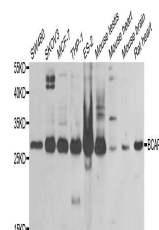
Western blot analysis of extracts of var...
