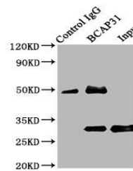
Immunoprecipitation analysis of Mouse li...
