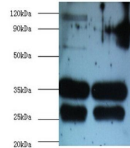
Western blot analysis of (Lane 1): EC109...
