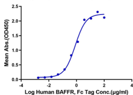
Biotinylated Human BAFF, His Tag ELISA 0.1 \mu g Biotinylated Human BAFF, His Tag Per Well
