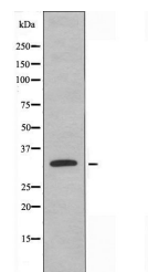
Western blot analysis of 293 cells, Jurk...
