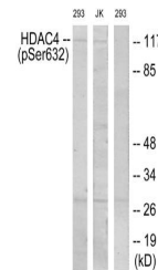
Western blot analysis of 293 cells and J...
