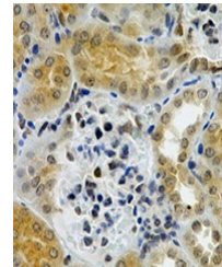
Immunohistochemical analysis of nNOS staining...
