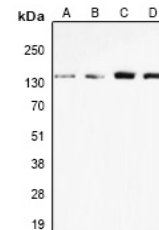
Western blot analysis of nNOS expression...
