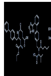
Chemical structure of AHU-377 ( LCZ696)
