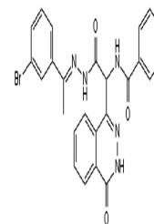
Chemical structure of AC 55541
