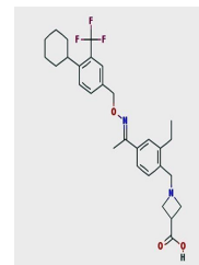
Chemical structure of BAF312 (Siponimod)
