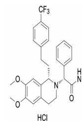
Chemical structure of Almorexant HCl (Ac...
